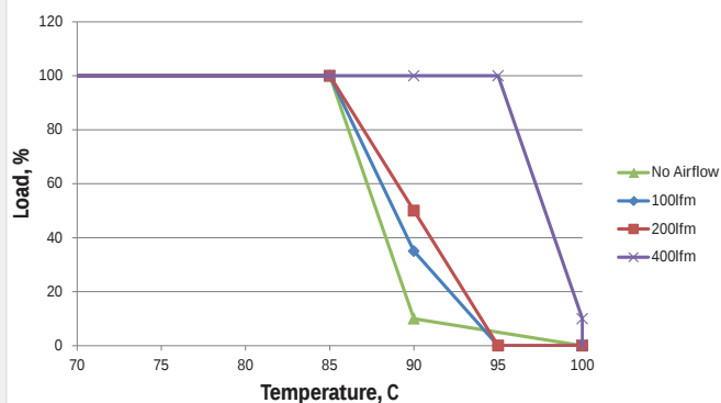
MTC1S1203MC - 18Vin
