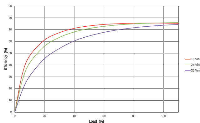
MTC1S2403MC
