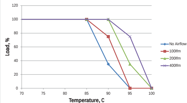
MTC1S2412MC - 18Vin
