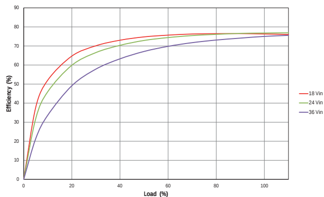
MTC1S2405MC
