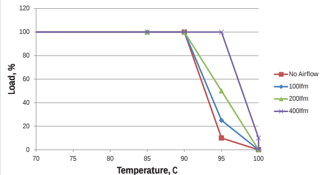
MTC1S2405MC- 24Vin
