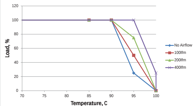
MTC1S2405MC - 18Vin
