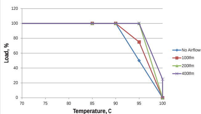
MTC1S2403MC - 18Vin
