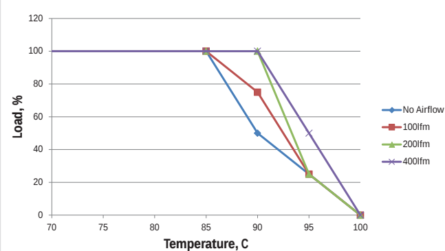
MTC1S2403MC - 18Vin
