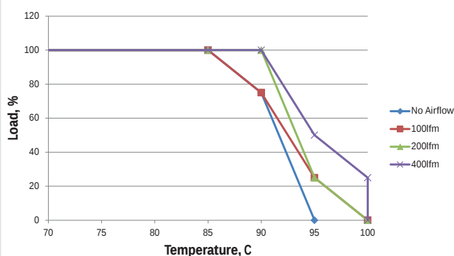
MTC1S1212MC - 9Vin
