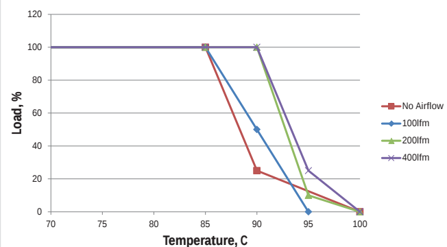
MTC1S2403MC- 24Vin
