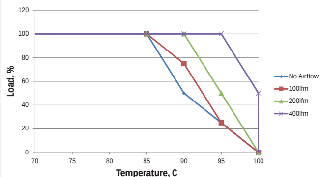
MTC1S1203MC - 9Vin
