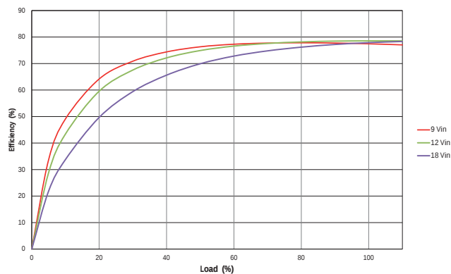
MTC1S1205MC
