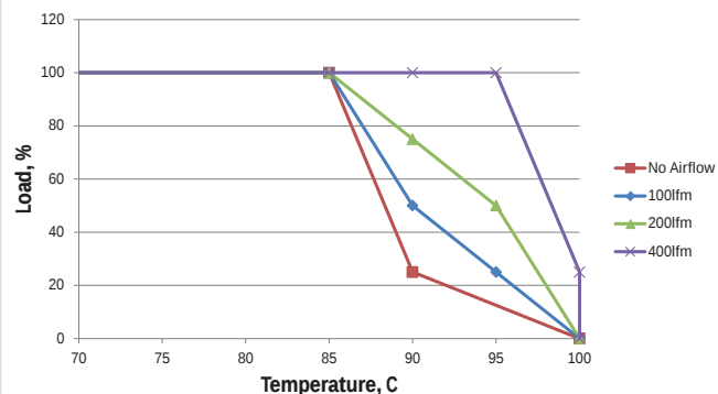
MTC1S1203MC - 12Vin
