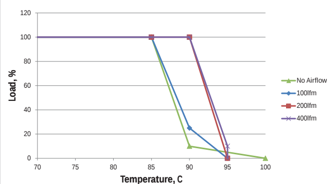
MTC1S2403MC- 36Vin
