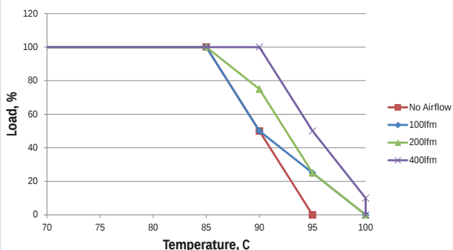
MTC1S1212MC- 12Vin
