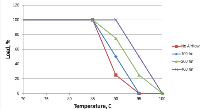
MTC1S2412MC- 24Vin
